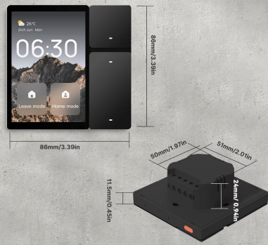
Zigbee Gateway panel Size (TLP03-C2 3.5 inch gateway panel)
